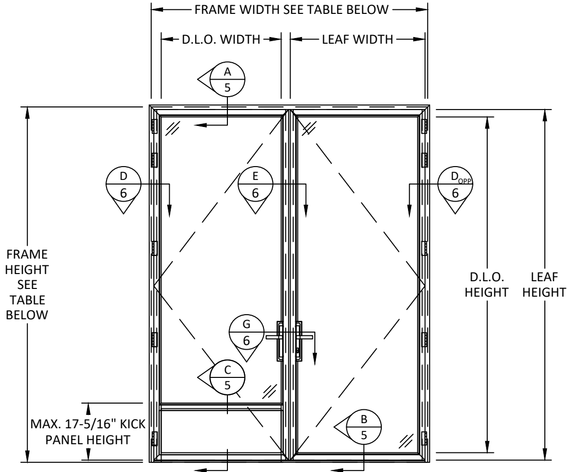
TYPICAL ELEVATION FRENCH DOOR
