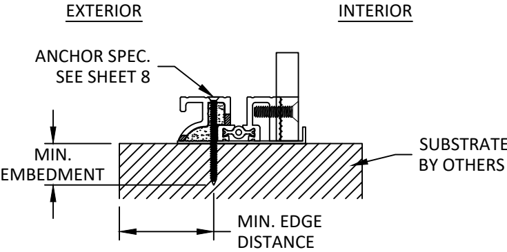
K 7 INSTALLATION DETAILS SILL SHOWN
