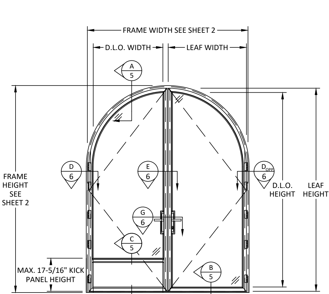
TYPICAL ELEVATION FRENCH DOOR, ROUND TOP
