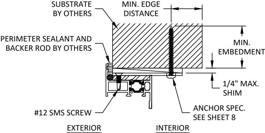
I 7 INSTALLATION DETAILS HEAD SHOWN, JAMB SIMILAR ANCHOR THROUGH STRAP ONLY
